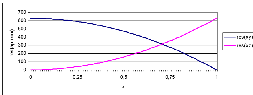
Fig. 6. Plotting the resolution of the of XY and XZ groups in dependency of the z -values.
